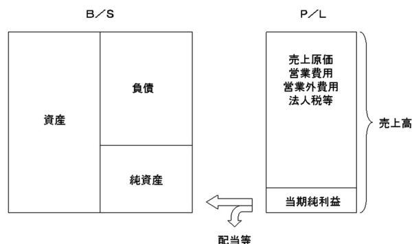
図1 B/SとP/L
